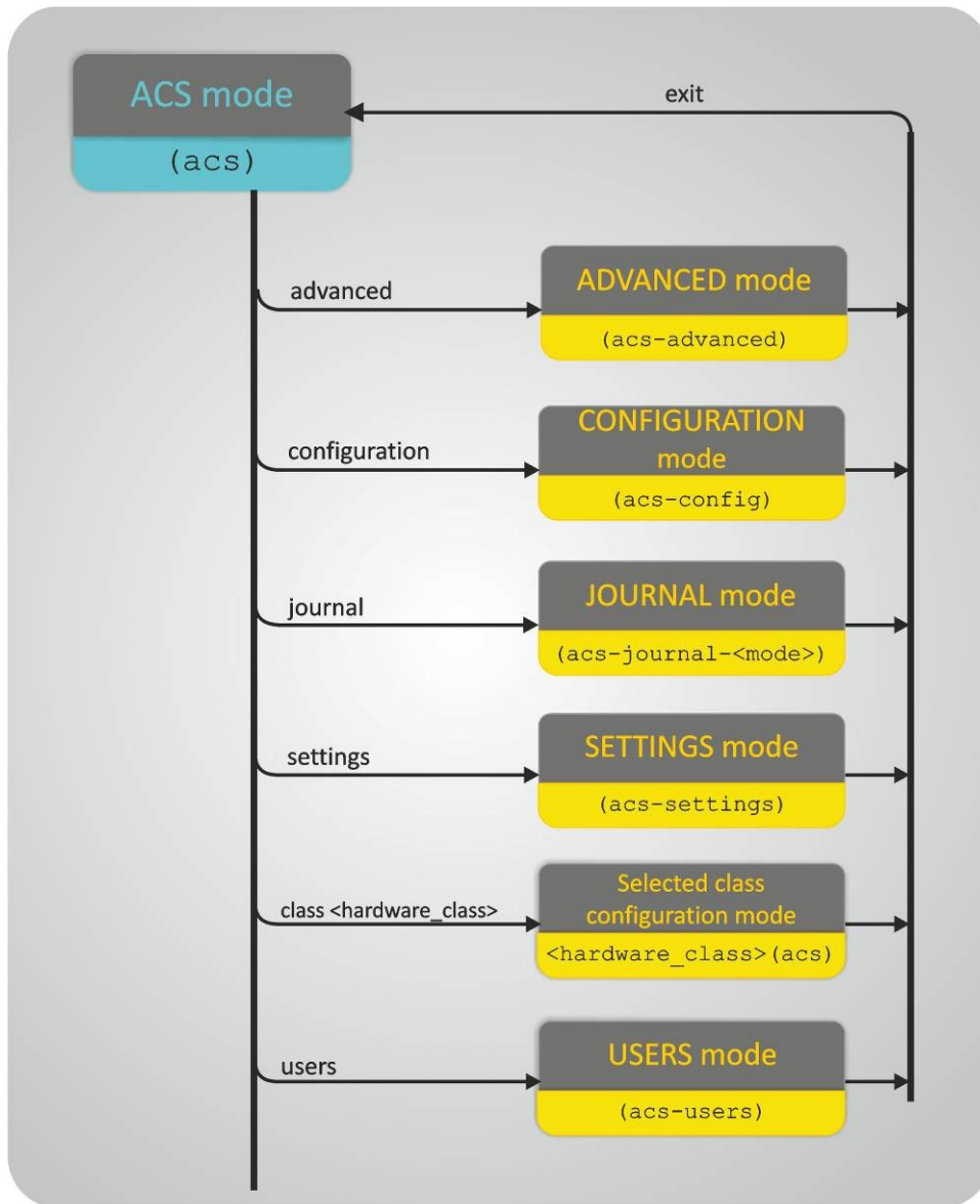
Fig. 1—Command mode hierarchy of the 'acs' block
