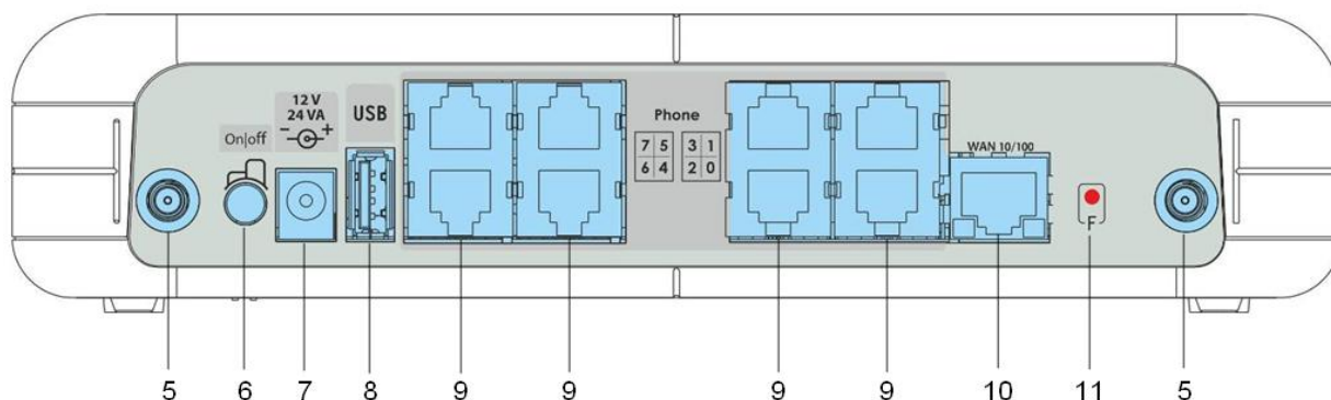
Fig. 5 – TAU-8.IP-W rear panel
